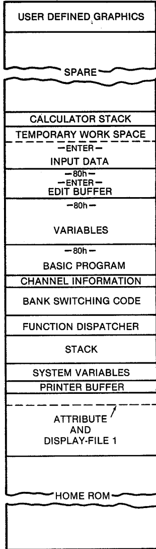
Fig. 5-2. Home Bank memory map (Numbers in parenthesis represent initial values for system variables — these will change as computer is used.)
